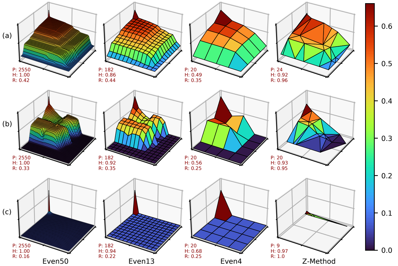
Fig. 4: Examples of point selection on 2-tier MRCs that highlight three different commonly observed scenarios. Each point represents the total miss ratio of a configuration of some L1 and L2 sizes. The x and y axes are the normalized L1 and L2 sizes, respectively, while the z -axis is the miss ratio. Axis labels are omitted to reduce clutter. Each row contains MRCs of a single workload using 4 different point-selection methods, listed at the bottom of each column. The P value indicates the total of number of points (lower is better), H is the HyperVolume as a percentage of Even50 (higher is better), and R is the Ratio of Non-Dominated Individuals (higher is better).
